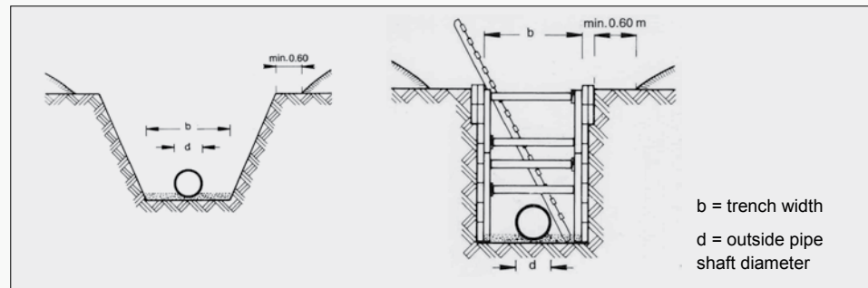
Fig. 4. Sloped & sheeted trenches
